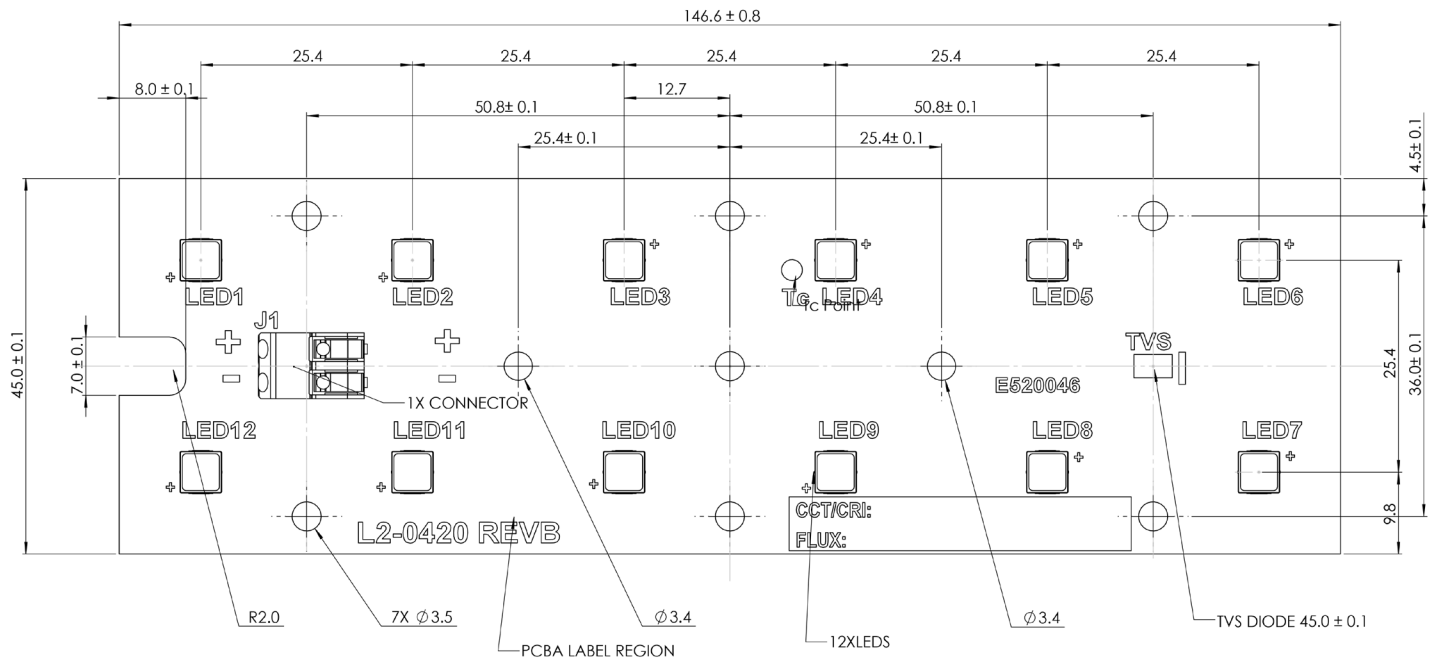
Top View
